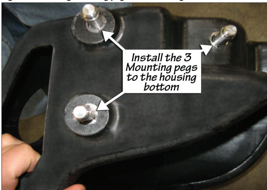
Figure 5- Attaching mounting pegs to the housing bottom
