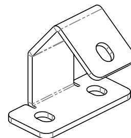
27 x2 Rail Support Bracket
