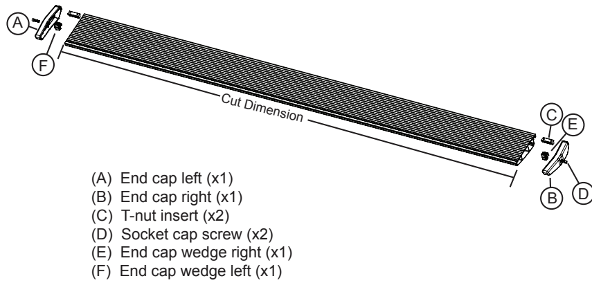
Running board assembly
