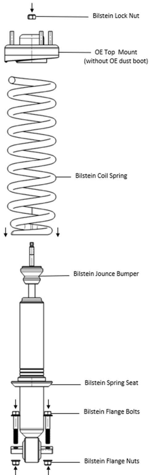
Figure 4: Assembly
