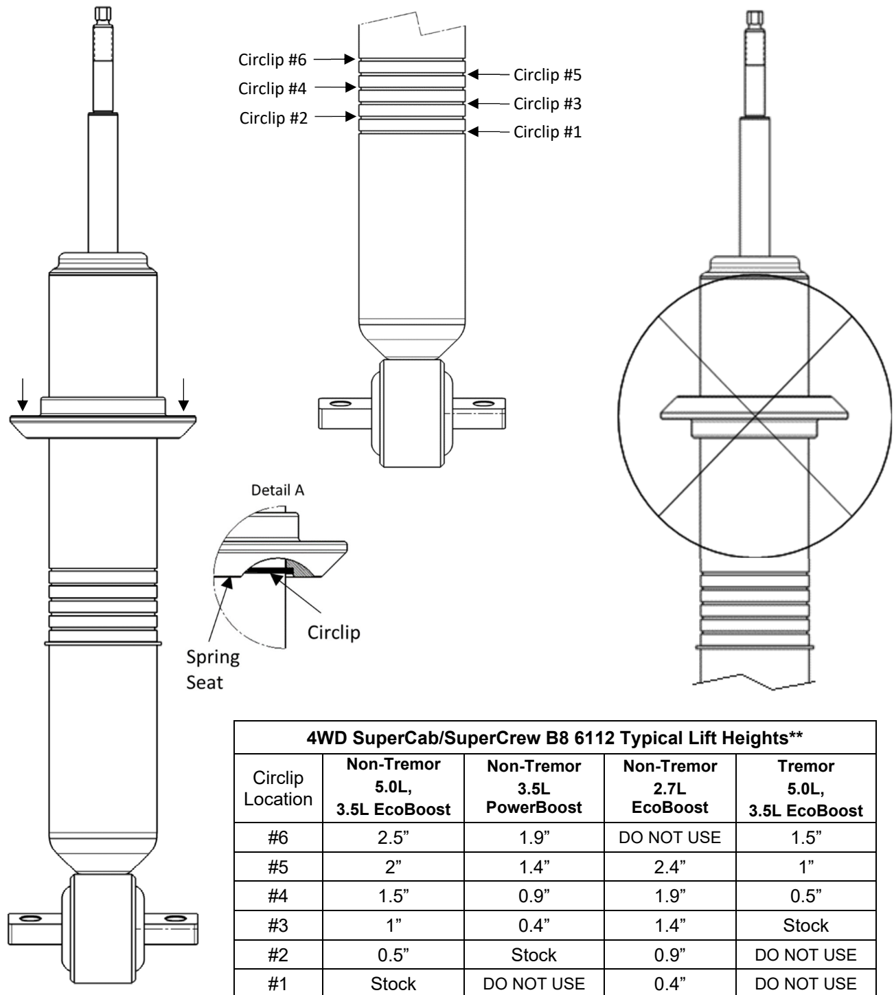
Figure 1: Circlip Location and Lift Heights
